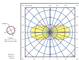
Courbe - SAH25I-V.125.70L
